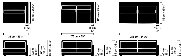
element 135 x 115 arm L/R
