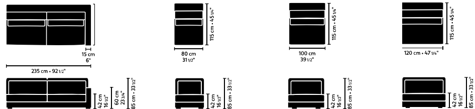
element 235 x 115 arm L/R
